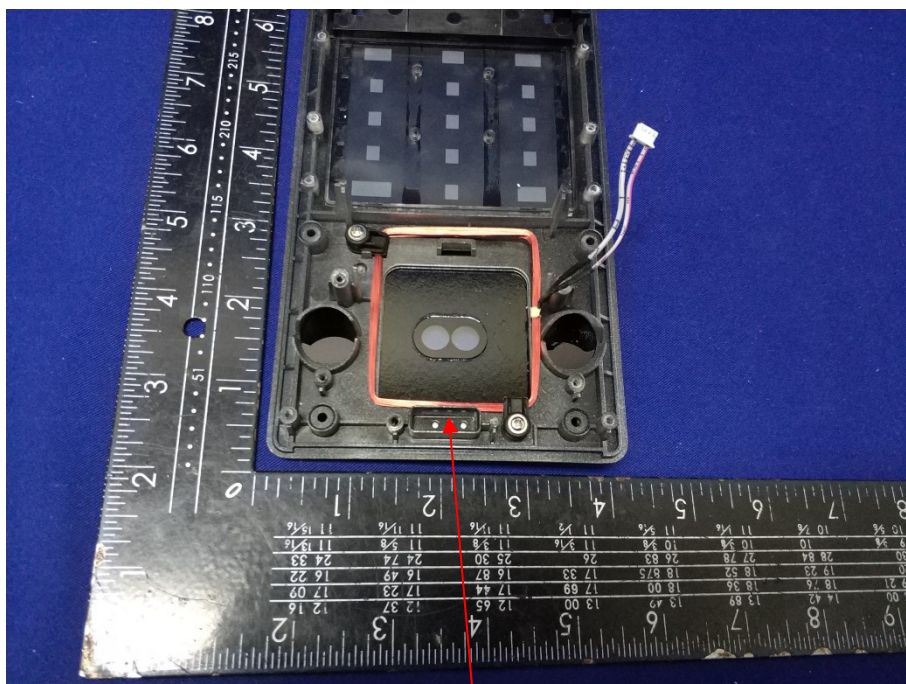
125KHz Antenna
