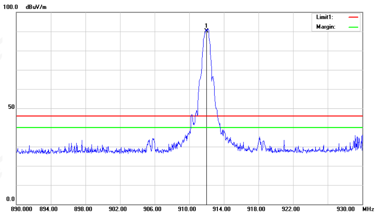
Fundamental Frequency
