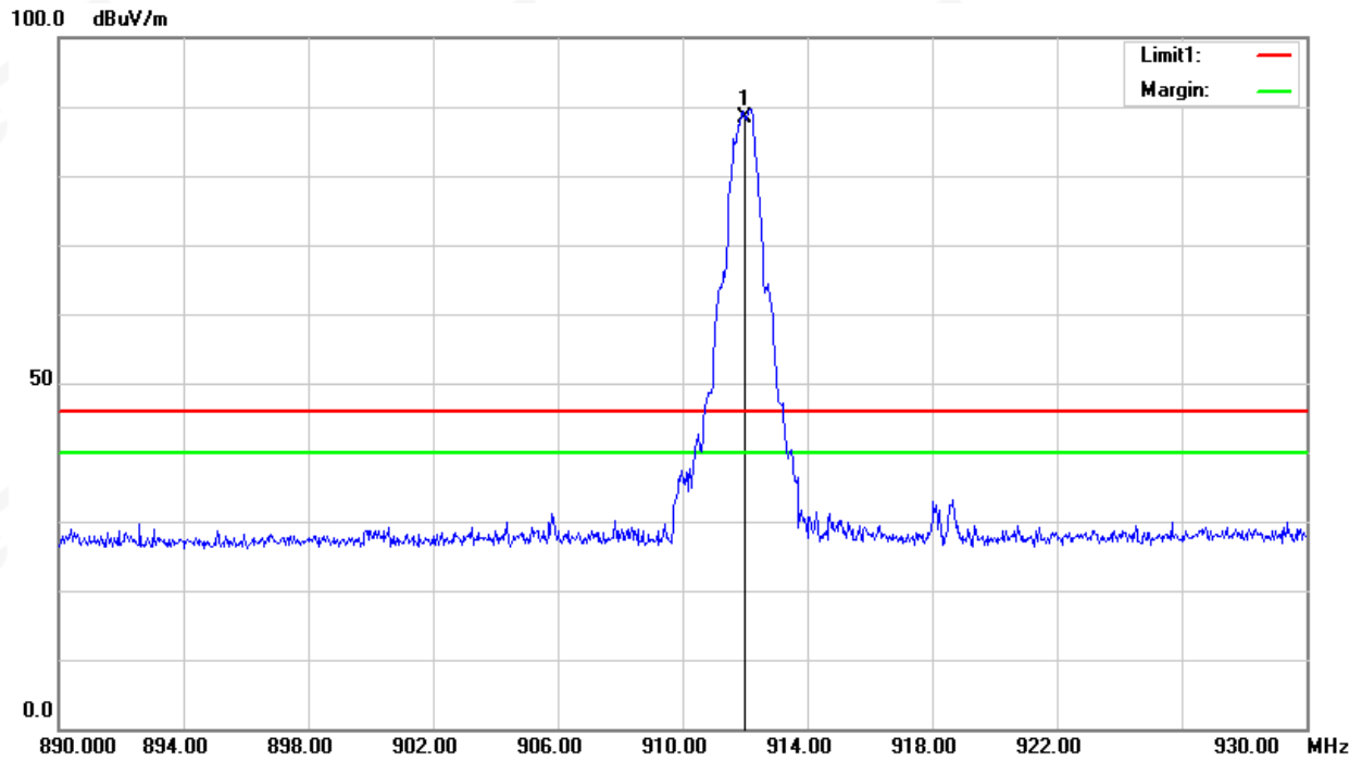
Fundamental Frequency
