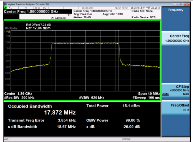
LCH_16QAM_100RB#0
