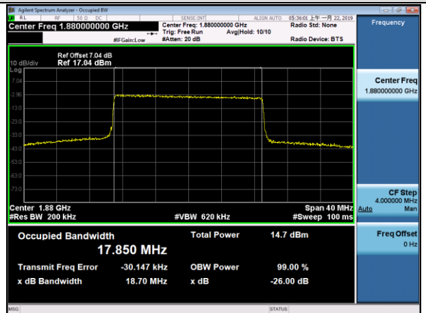
MCH_16QAM_100RB#0
