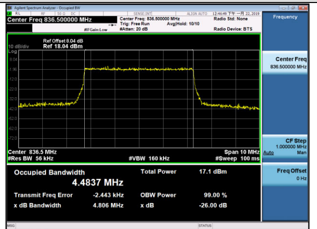
MCH_16QAM_25RB#0
