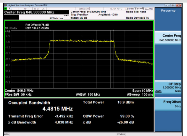
HCH_16QAM_25RB#0
