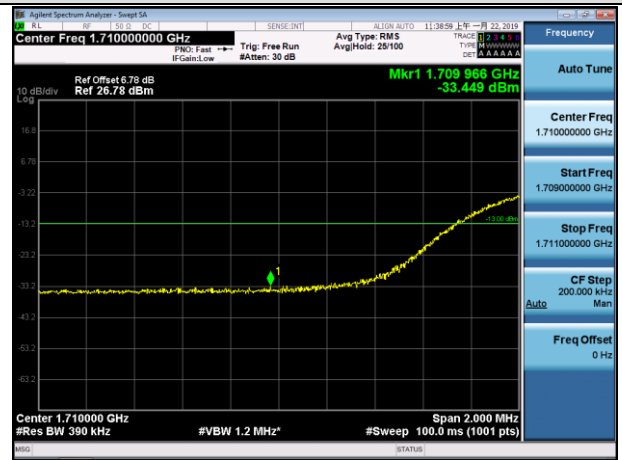
LCH_16QAM_100RB#0
