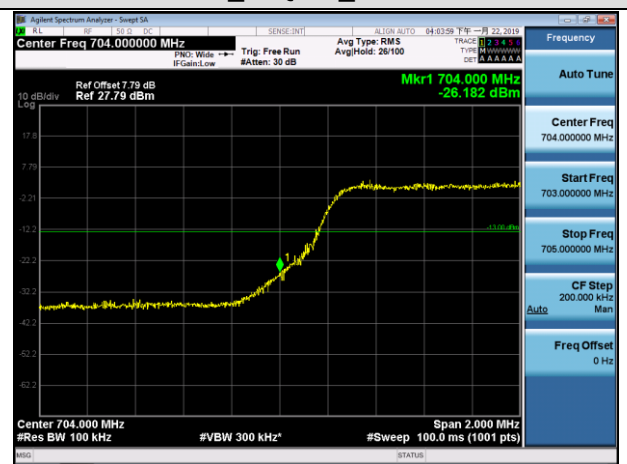
LCH_16QAM_25RB#0
