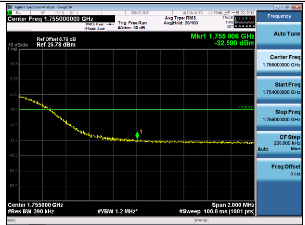
HCH_16QAM_100RB#0
