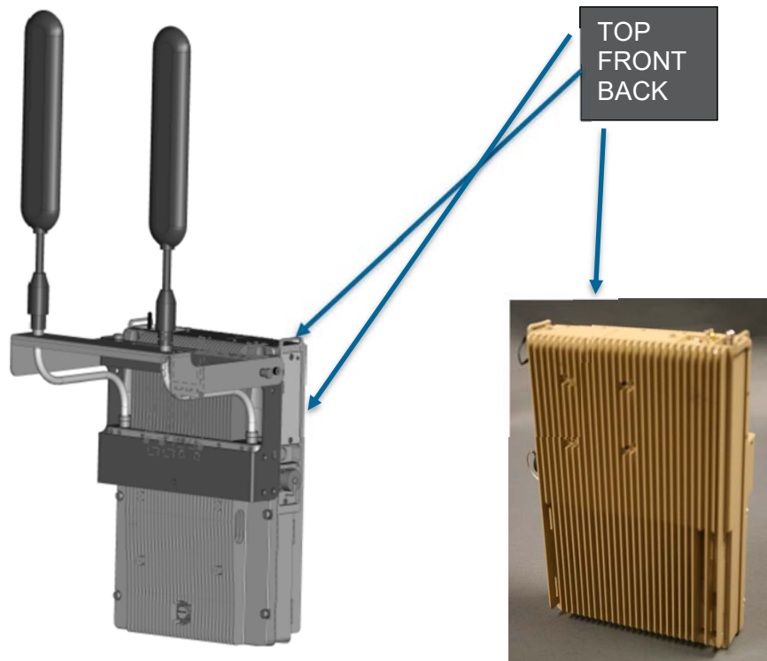
Figure 1: Xiphos Micro
