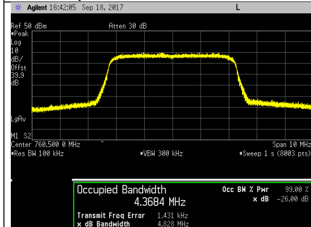
LTE - 5M - 16QAM - Low Channel
