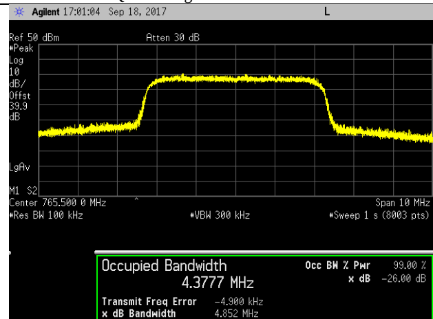
LTE - 5M - 64QAM - High Channel
