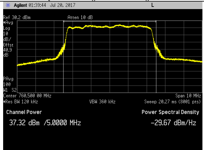
Port 1 - LTE - 16QAM - 5M - High Channel - Average
