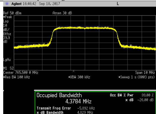
LTE - 5M - 16QAM - High Channel
