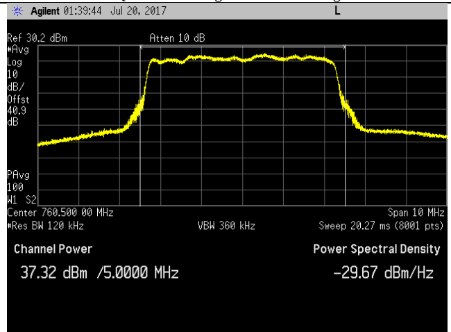
Port 1 - LTE - 64QAM - 5M - High Channel - Average
