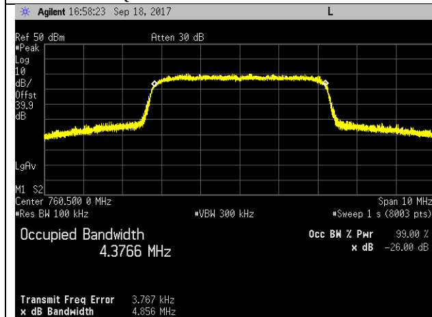
LTE - 5M - 64QAM - Low Channel
