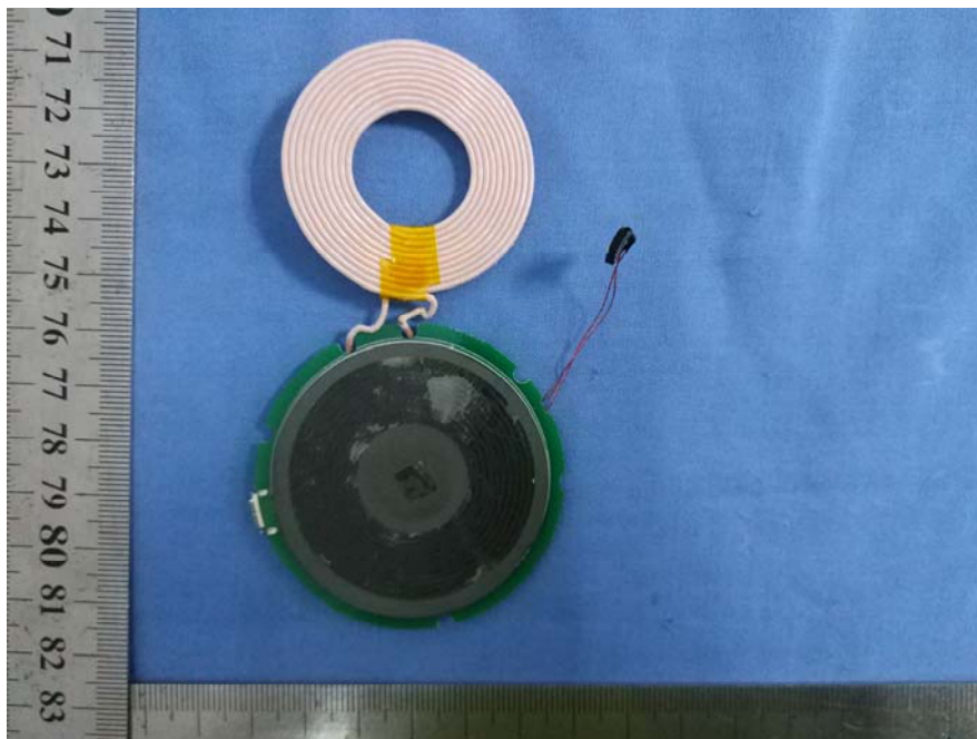
EUT – Loop Inductive Antenna View
