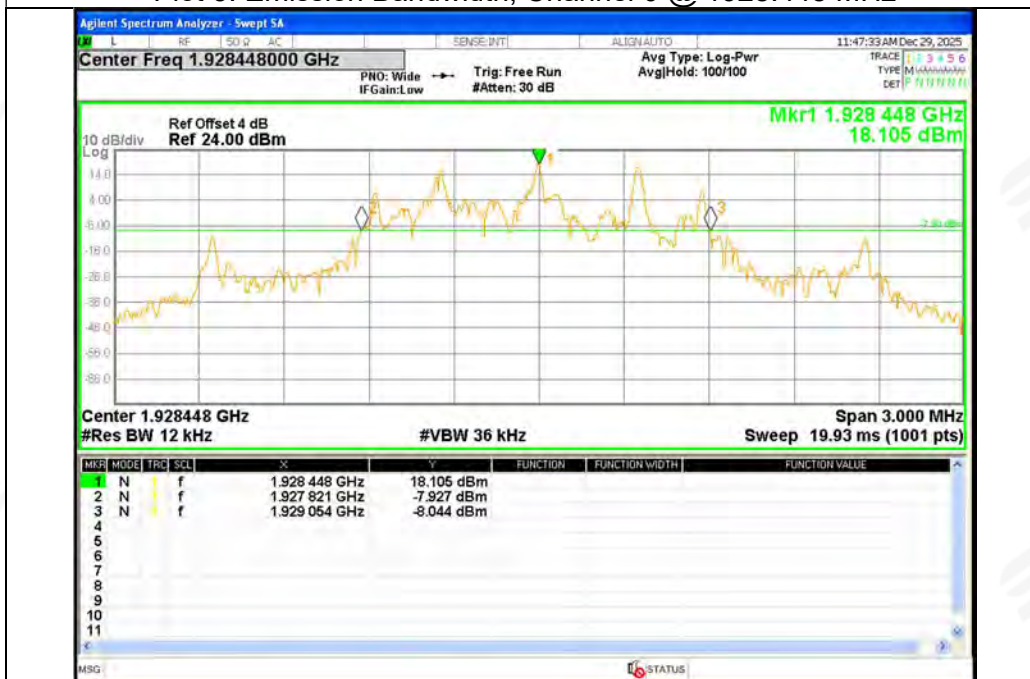
Plot 3. Emission Bandwidth, Channel 0 @ 1928.448 MHz
