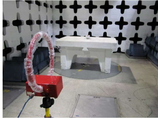
Radiated emissions test set up below 30MHz.
