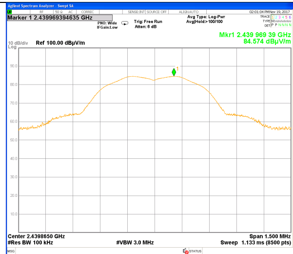
Plot # 8. Carrier frequency – 2440 MHz
