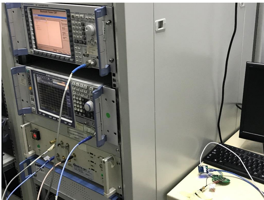
Conducted Test-BT3.0
