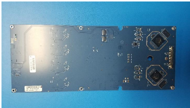
830-00010_REV4_RBK6028_mmwSURF_BOT
