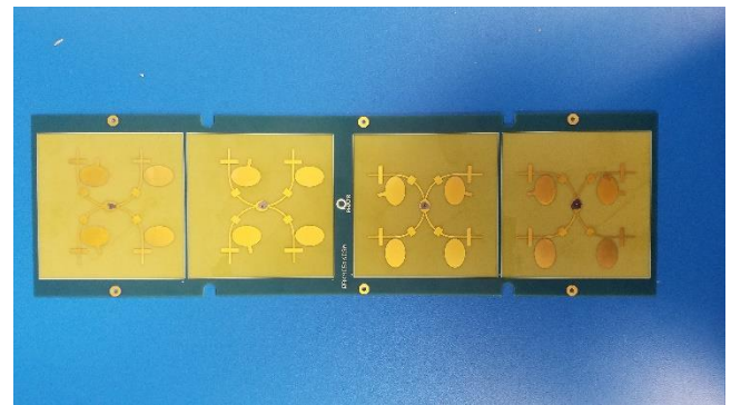
170-00014_REV1_RBK60xx_sub6SURF_ANTENNA_TOP
