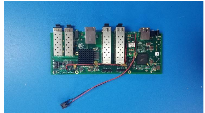
820-00028_REV1_RBK60xx_SWITCH_TOP
