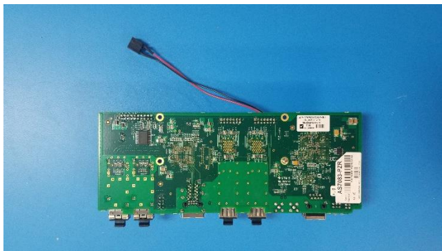
820-00028_REV1_RBK60xx_SWITCH_BOT
