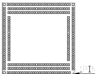
Figure 1-5. Bottom View
