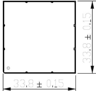
Figure 1-3. Top View
