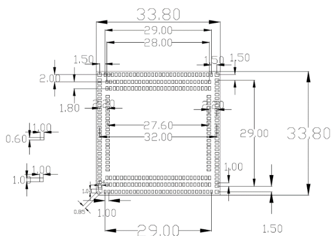
Figure 1-6. Package Dimensions
