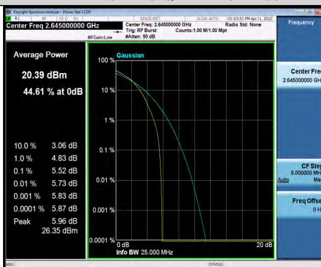
Band41-20MHz-64QAM-41140-100RB#0
