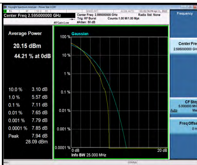
Band41-20MHz-64QAM-40640-100RB#0
