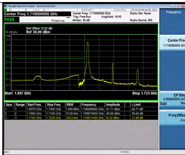
Band66-10MHz-64QAM-132022-50RB#0
