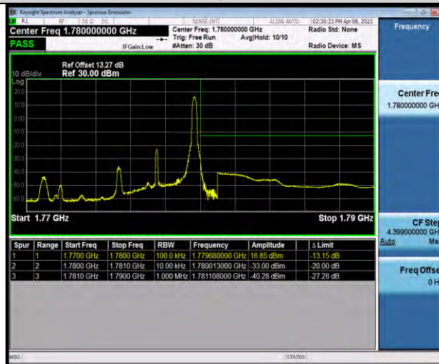
Band66-5MHz-64QAM-132647-25RB#0
