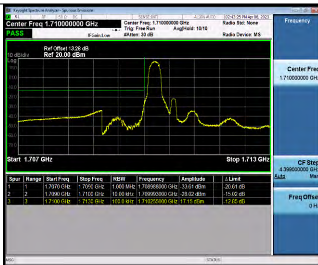
Band66-1.4MHz-64QAM-131979-6RB#0
