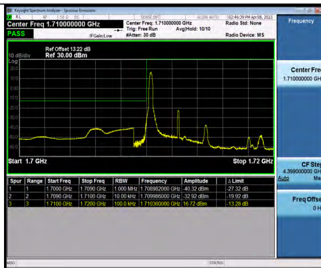
Band66-5MHz-64QAM-131997-25RB#0
