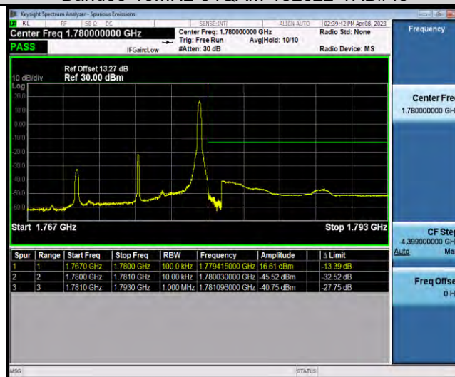
Band66-10MHz-64QAM-132622-50RB#0
