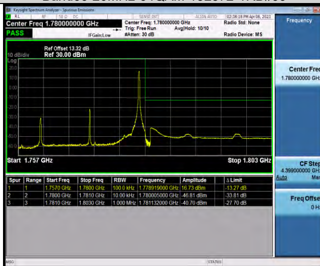
Band66-20MHz-64QAM-132572-100RB#0
