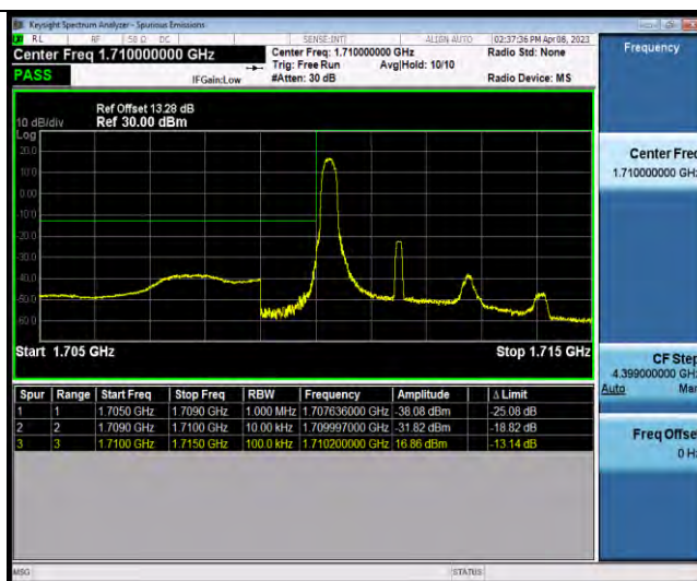
Band66-3MHz-64QAM-131987-15RB#0
