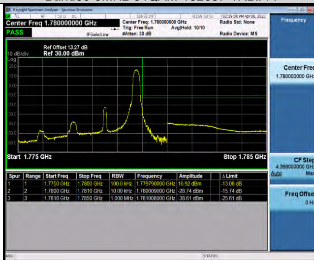
Band66-3MHz-64QAM-132657-15RB#0
