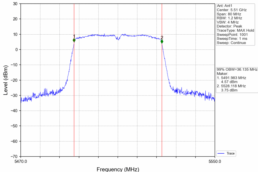
802.11ac(VHT40)_LCH_5510MHz_Ant1_NTNV
