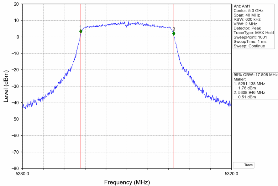
802.11ac(VHT20)_MCH_5300MHz_Ant1_NTNV
