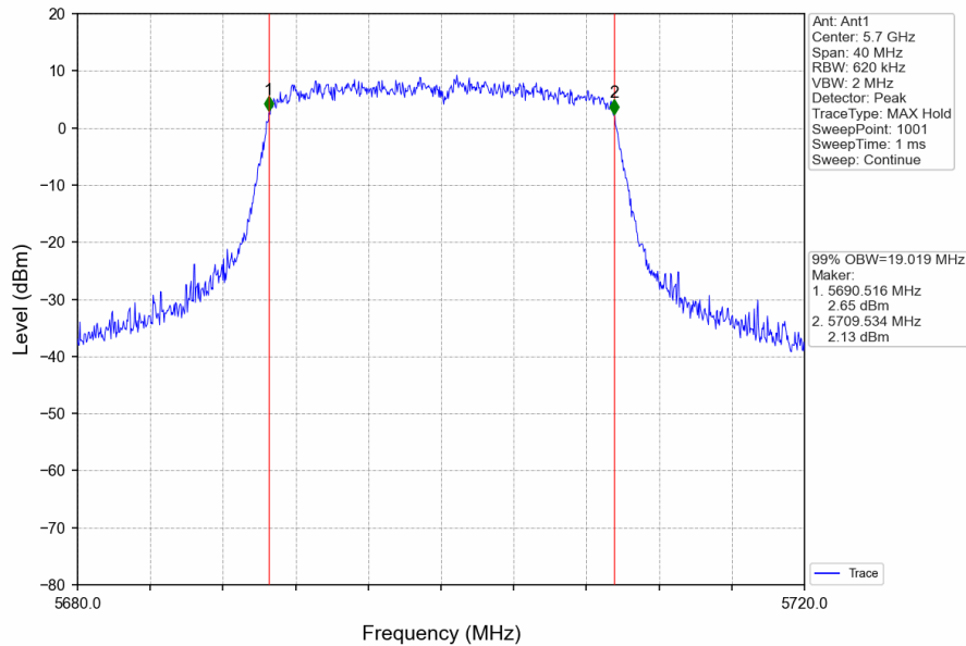
802.11ax(HEW20)_HCH_5700MHz_RU242_Left_Ant1_NTNV
