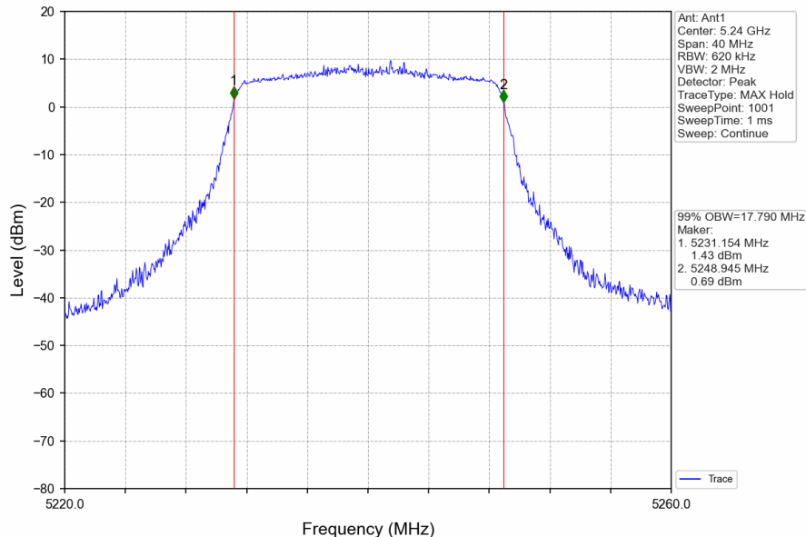
802.11ac(VHT20)_HCH_5240MHz_Ant1_NTNV
