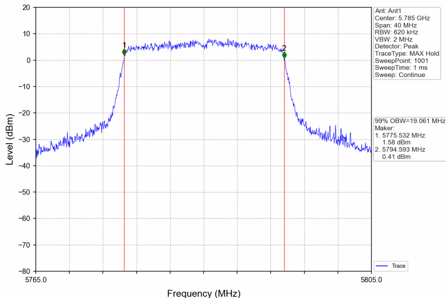
802.11ax(HEW20)_MCH_5785MHz_RU242_Left_Ant1_NTNV
