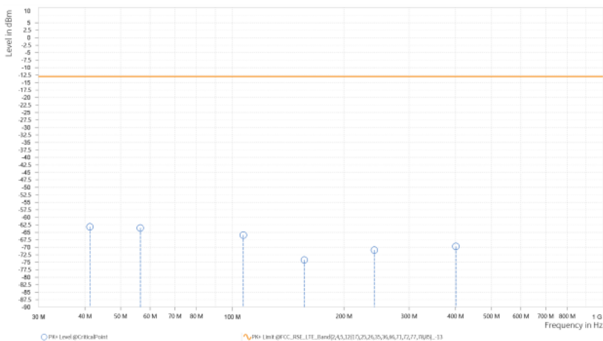
Spectrum Overview
