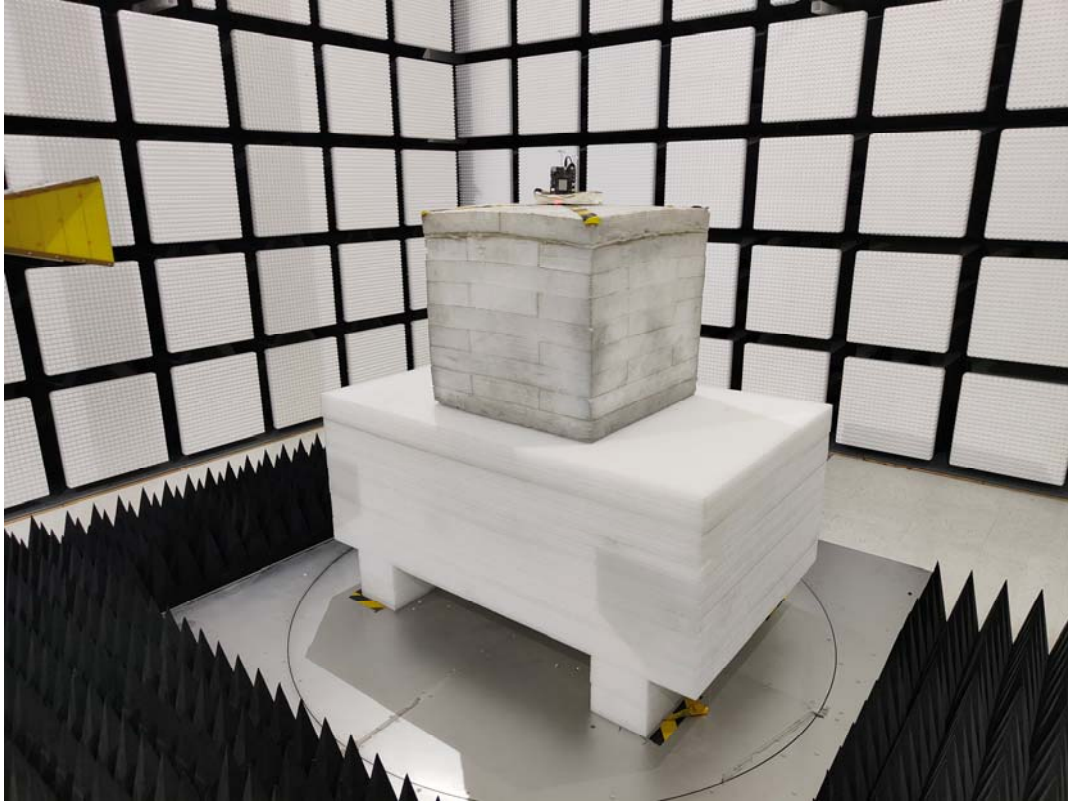
Radiated Emissions Above 1G View-FPC Antenna
