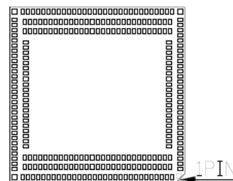
Figure 1-4. Bottom View
