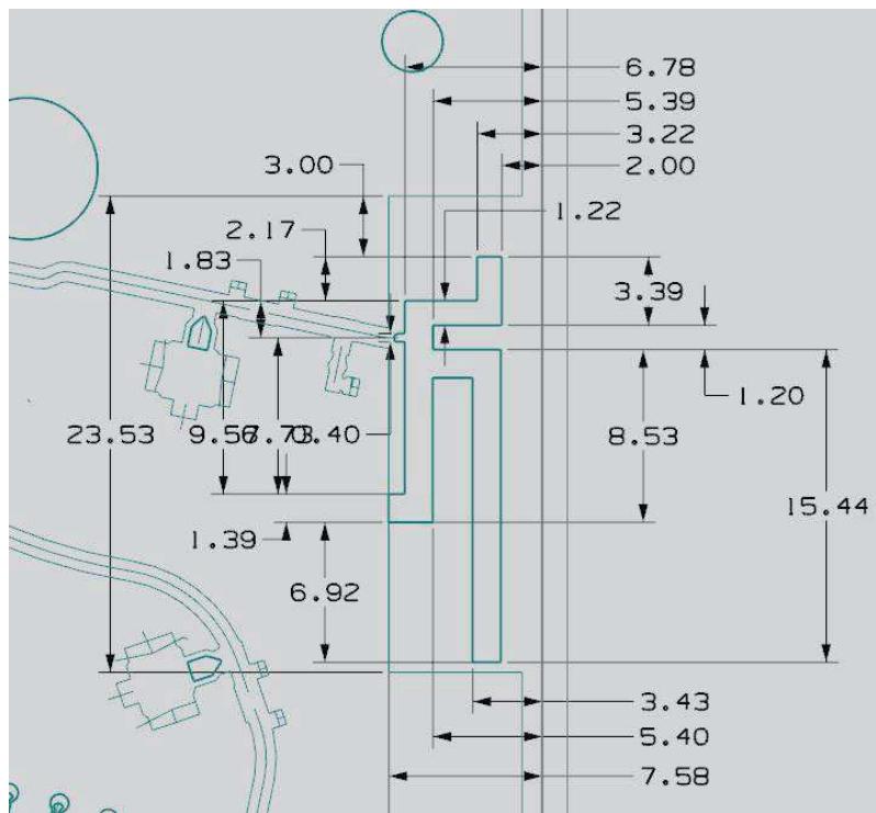
Antenna Pattern Detail – Ant-A2
