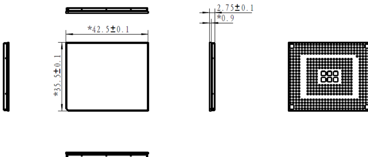
Figure 1-3. TurboX C6490 SOM Mechanical Dimensions
