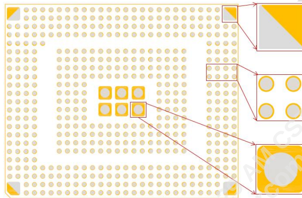
Figure 1-5. Stencil Aperture Diagram
