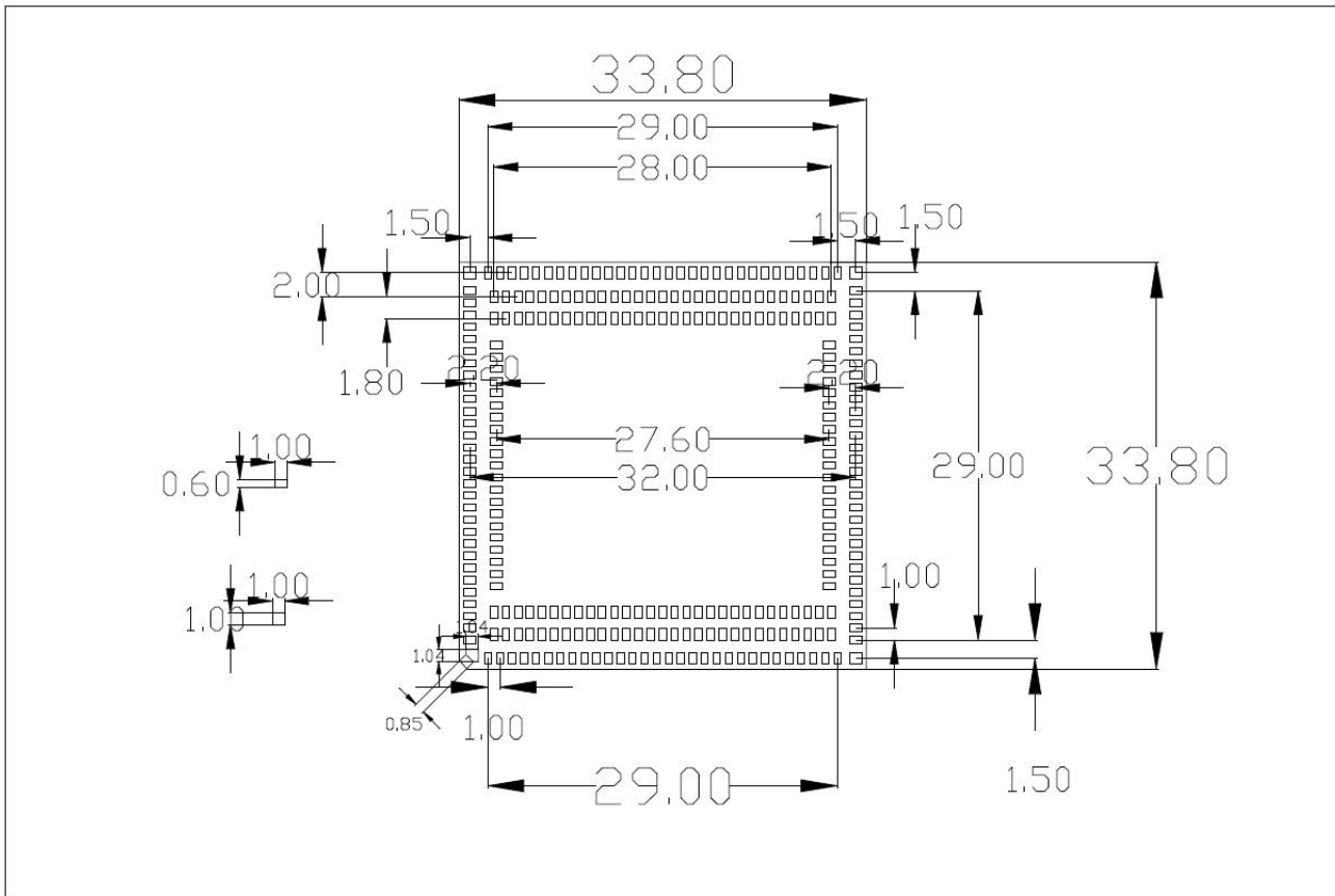
Figure 5-4 package dimensions
