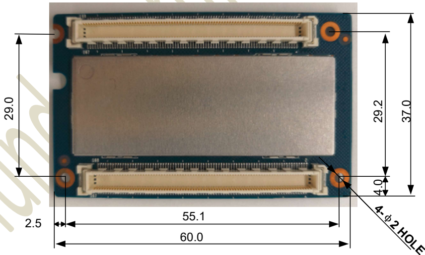
Figure 1.3-3 Bottom View
