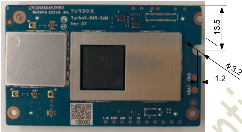
Figure 1.3-1 Top View
