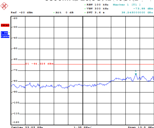
5800MHz 26.5GHz-40GHz
