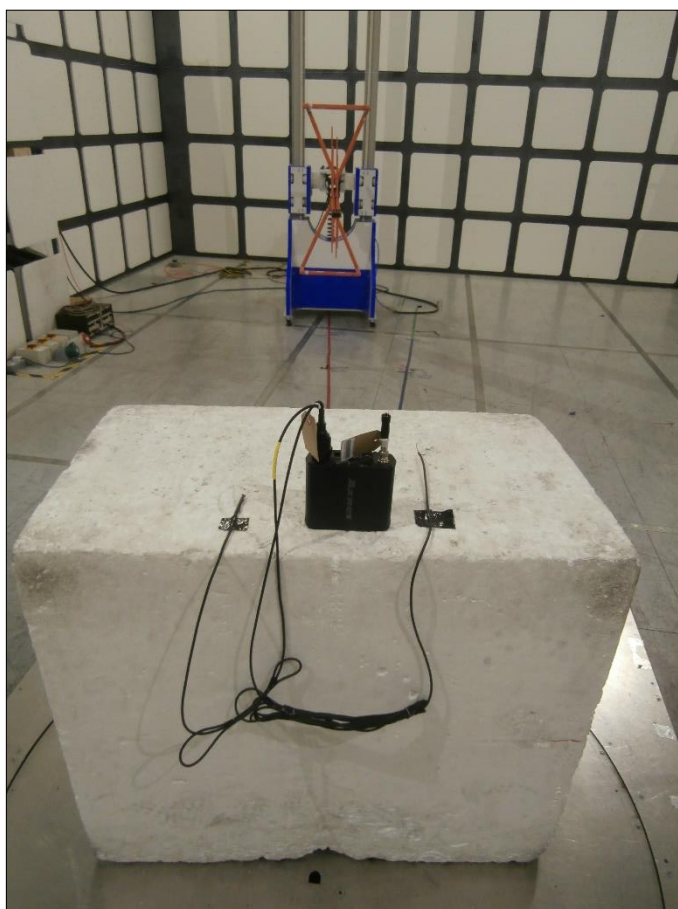
Figure 24 - Test Setup - 30 MHz to 1 GHz, Y Orientation
