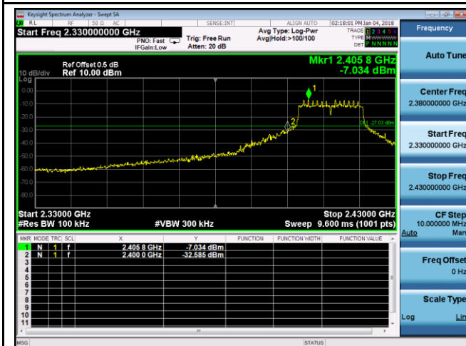
Band Edge, Left Side (Peak) - 802.11n20
