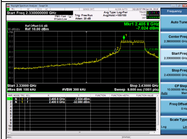
Band Edge, Left Side (Peak) - 802.11g
