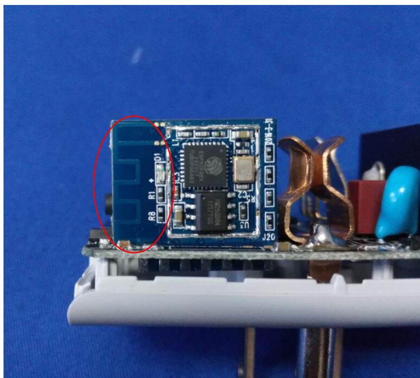
WIFI - Antenna View
