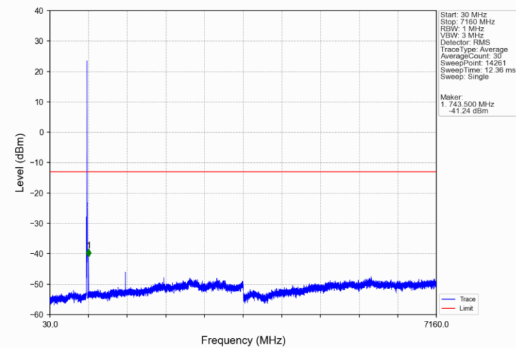
Band12_5MHz_16QAM_HCH_713.5MHz_RB_1_0_NTNV
