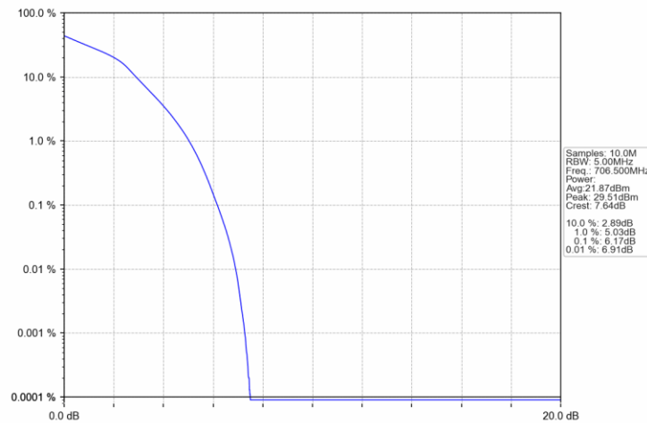
Band17 5MHz 16QAM LCH 706.5MHz RB 25 0 NTNV
