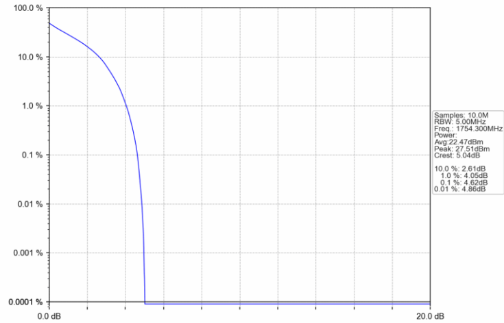
Band4_1.4MHz_QPSK_HCH_1754.3MHz_RB_6_0_NTNV
