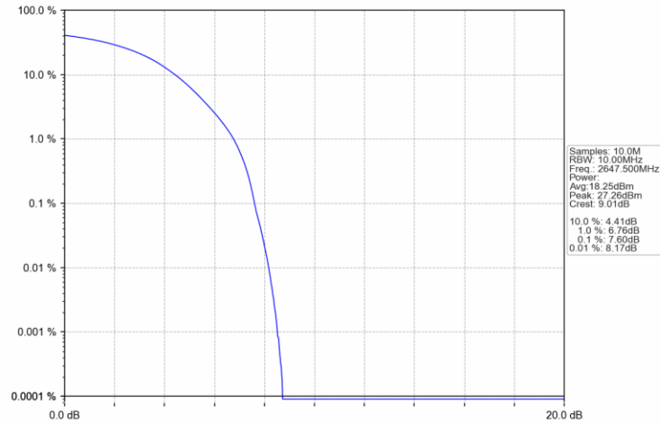
Band41_15MHz_QPSK_HCH_2647.5MHz_RB_75_0_NTNV
