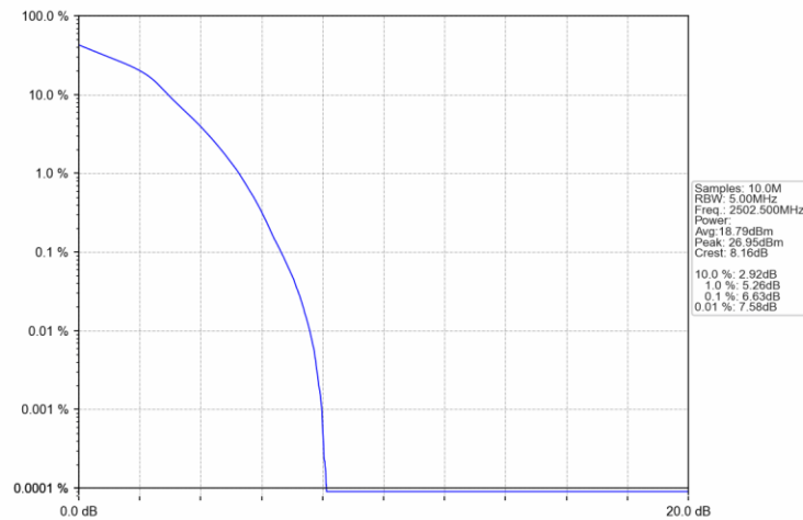
Band7 5MHz 16QAM LCH 2502.5MHz RB 25 0 NTN
