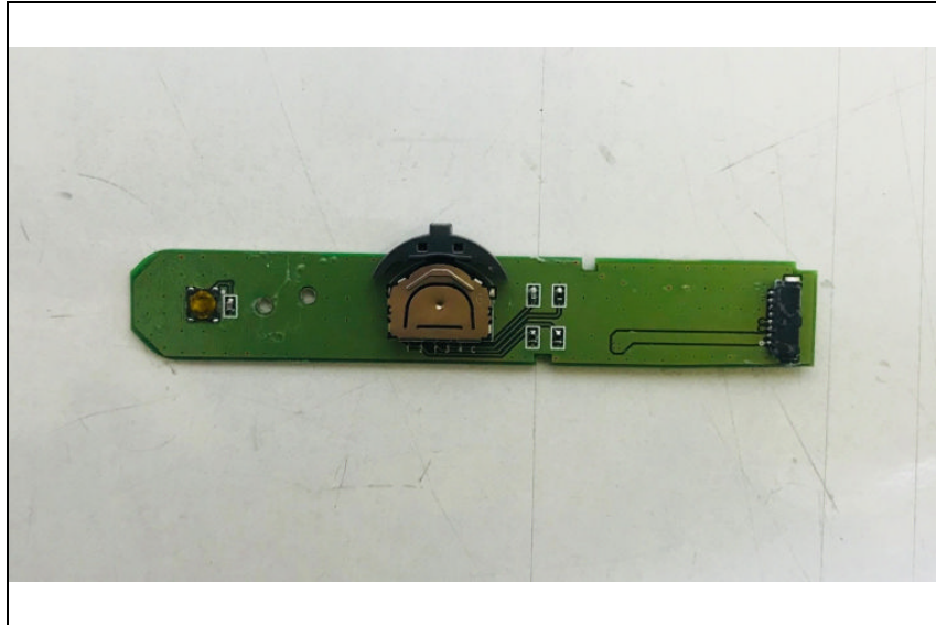
Bottom view of RIGHT PCB
