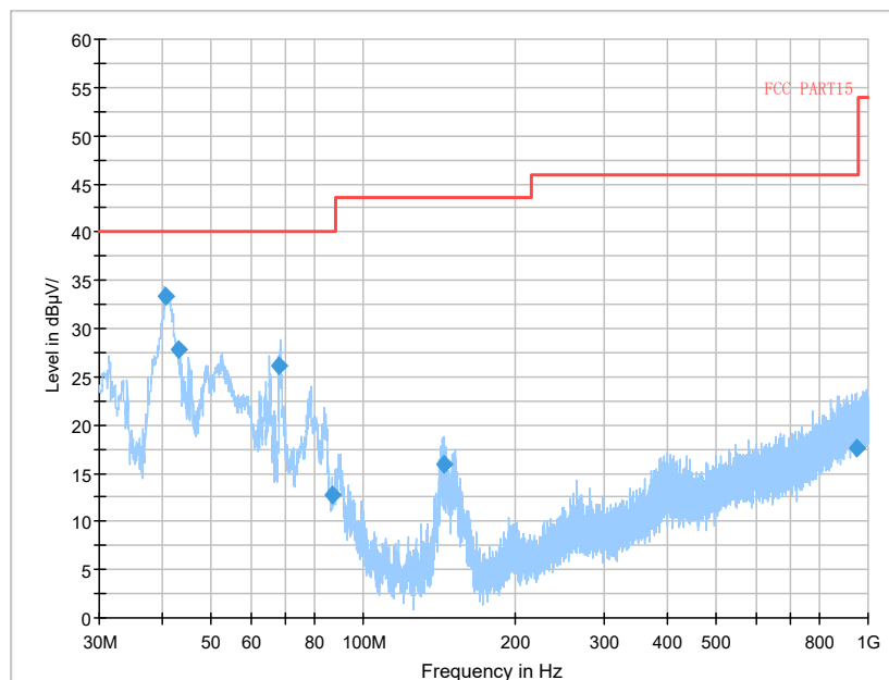
Frequency Range: 30MHz-1000 MHz Detector: QP mode Modulation type: GFSK (LE)
