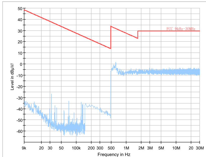
Frequency Range: 9kHz-30MHz Detector: QP mode Modulation type: GFSK (LE)
