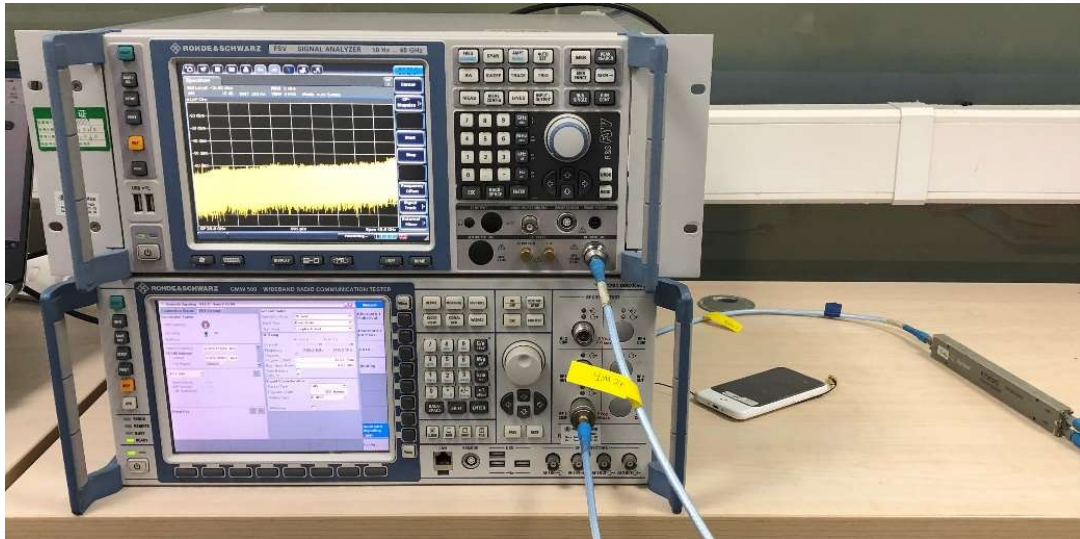
RF Conducted Test
