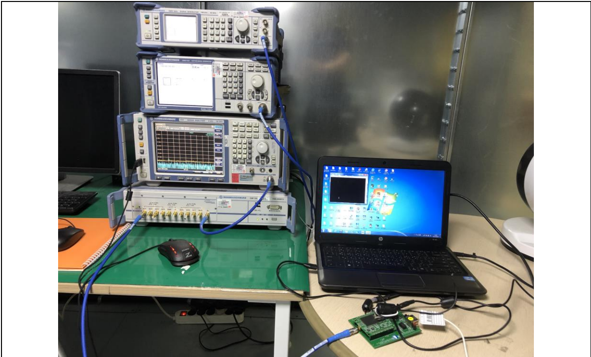
Test setup Photo
