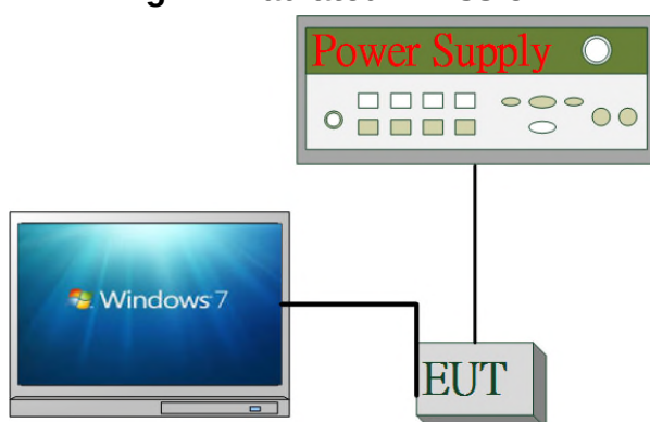
Fig 2-2 Radiated Emission
