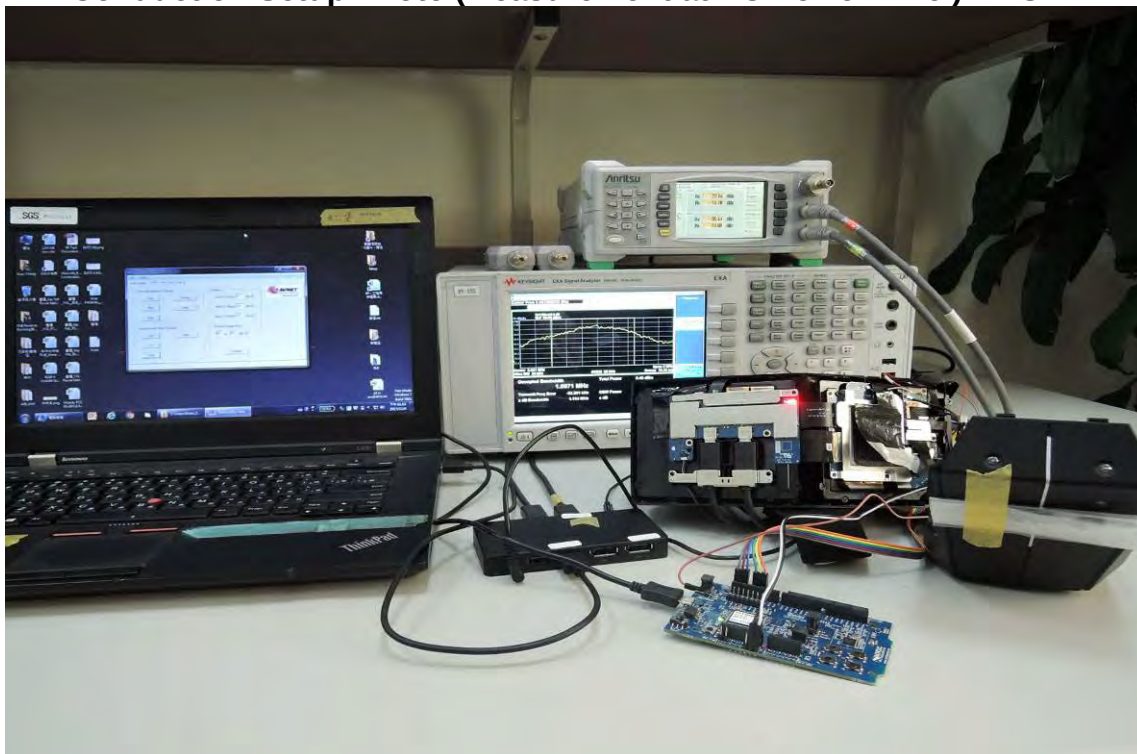
Conduction Setup Photo (Measurement at AC Power Line )-2.4GHz
