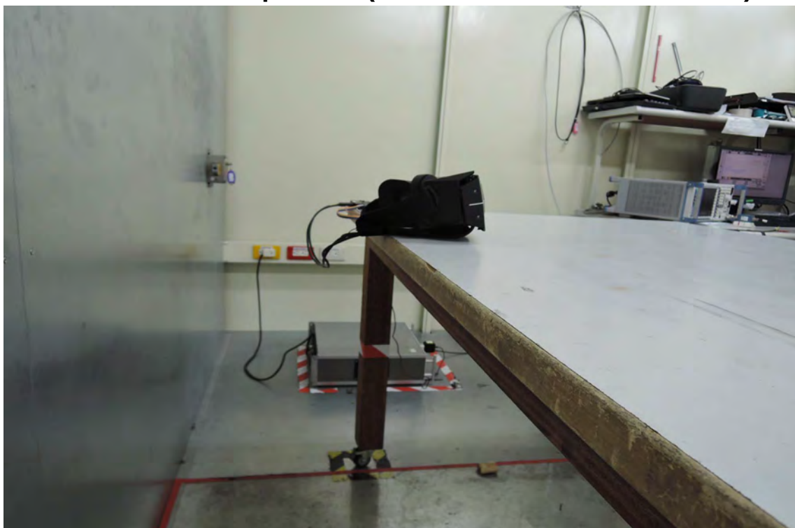
Conduction Setup Photo (Measurement at Antenna Port)
