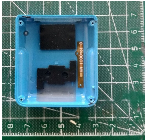
Figure 3: LEO top enclosure internal view
