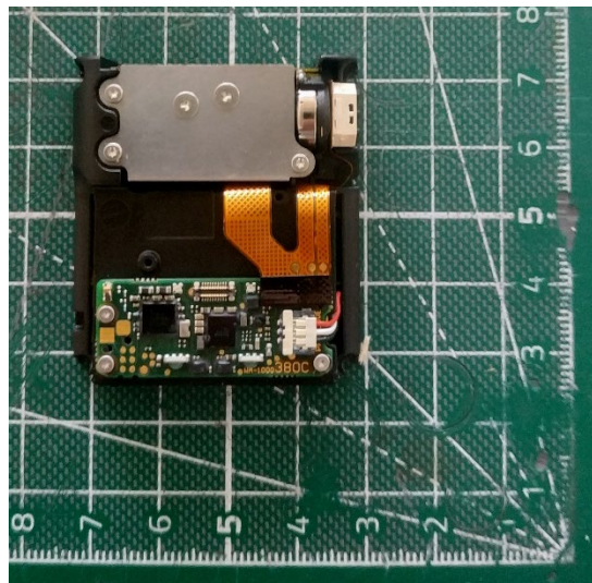
Figure 2: LEO internal top view
