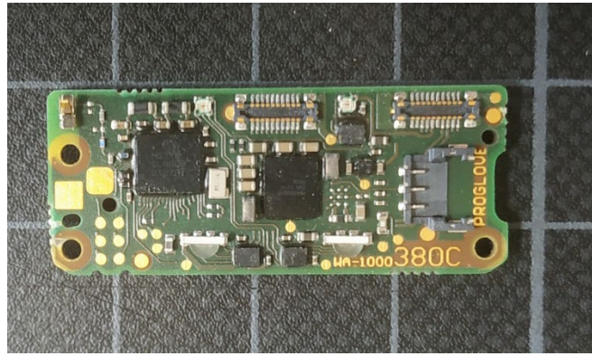
Figure 6: Top View,, Main PCB
