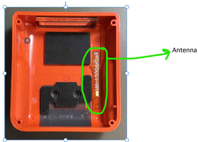
Figure 3: MARK 3 top enclosure internal view
