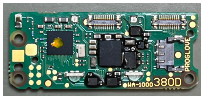
Figure 6: Top View,, Main PCB
