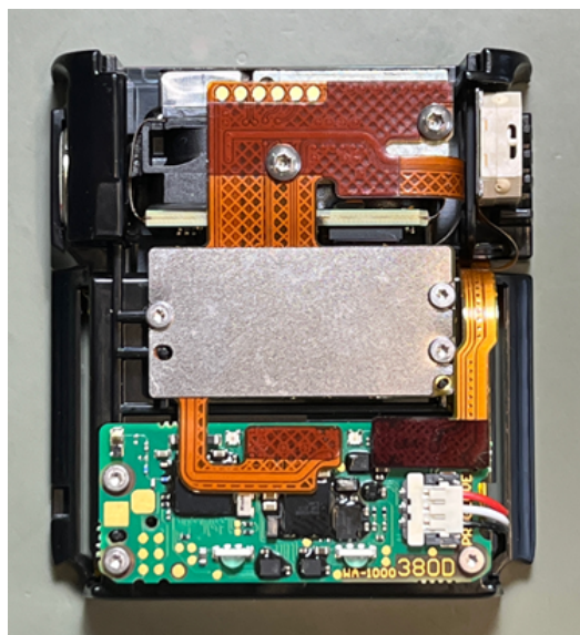
Figure 2: MARK 3 internal top view
