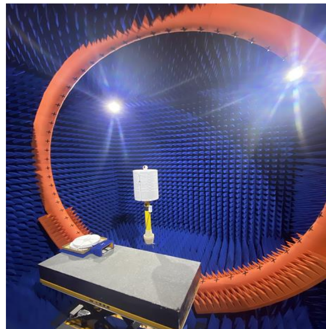
Testing 3D microwave darkroom(6m*6m*6m)
