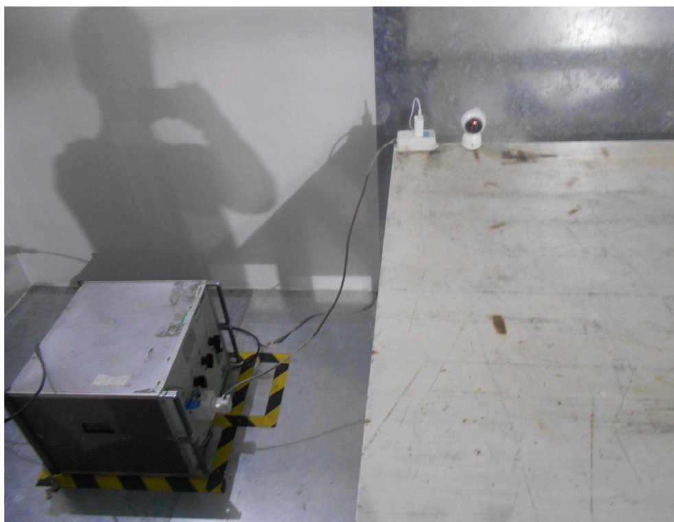
Conducted Emission
