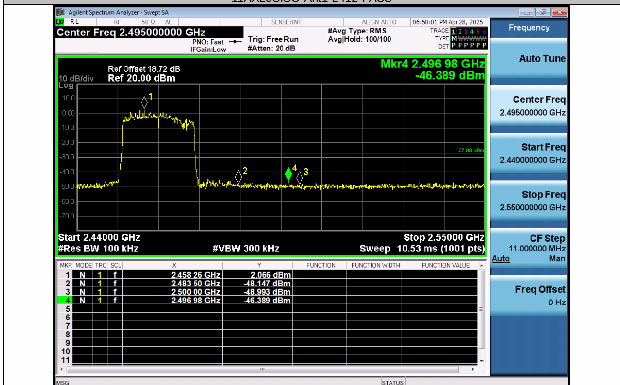
11AX20SISO-Ant1-2462-PASS
