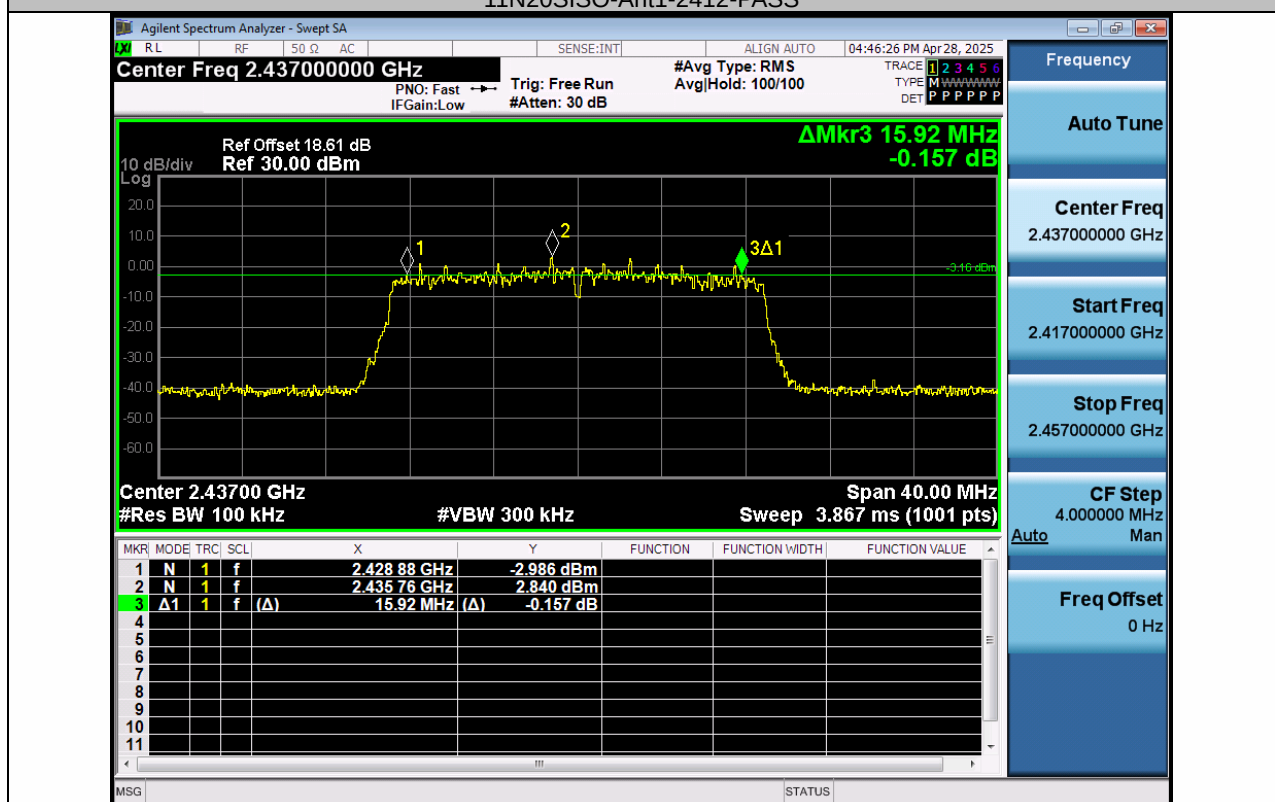
11N20SISO-Ant1-2437-PASS
