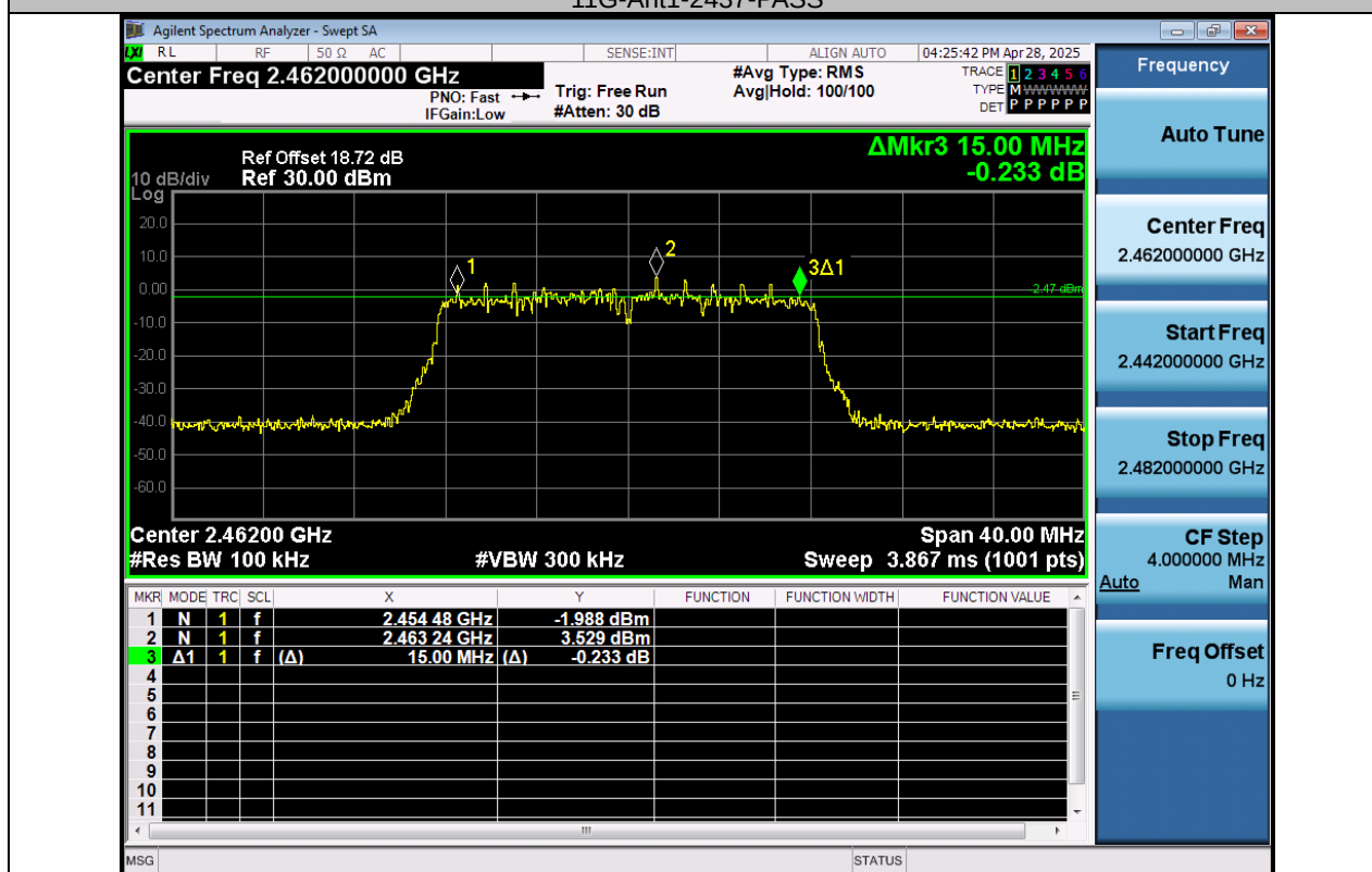
11G-Ant1-2462-PASS
