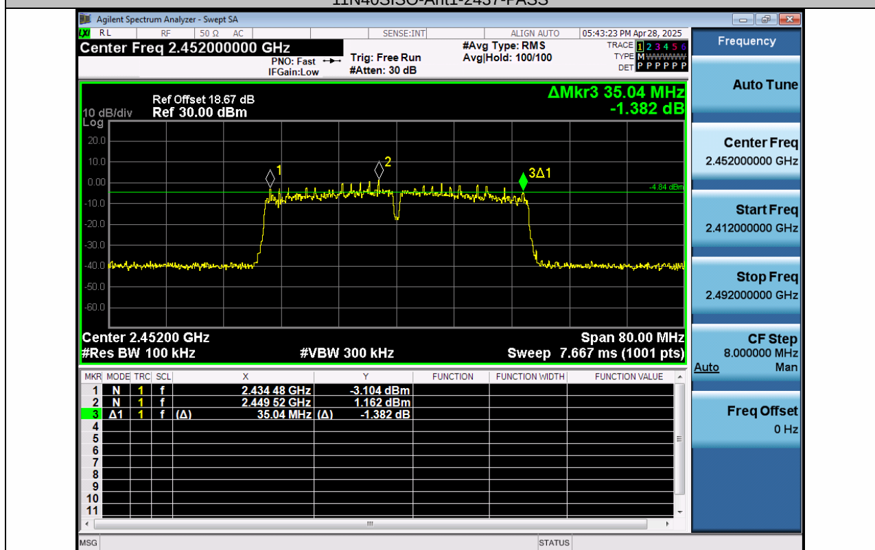
11N40SISO-Ant1-2452-PASS
