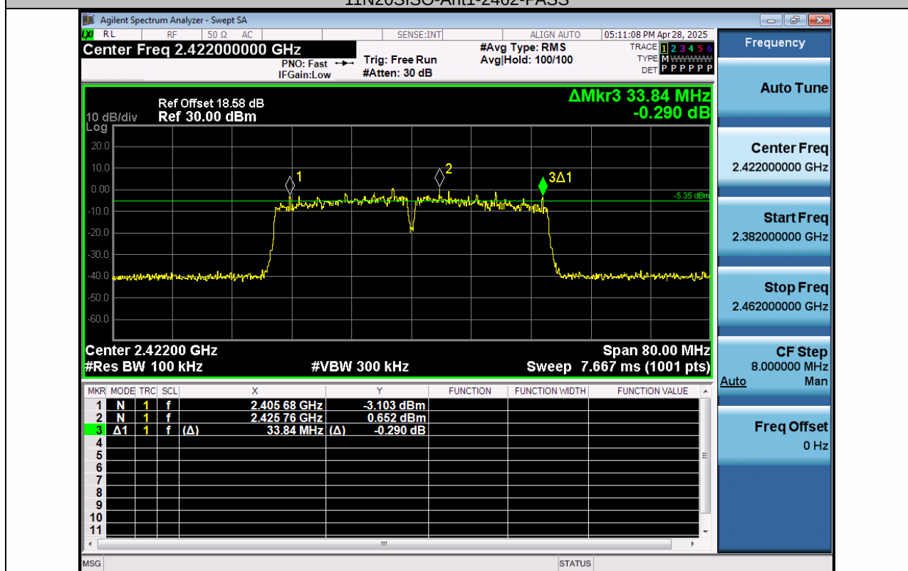
11N40SISO-Ant1-2422-PASS
