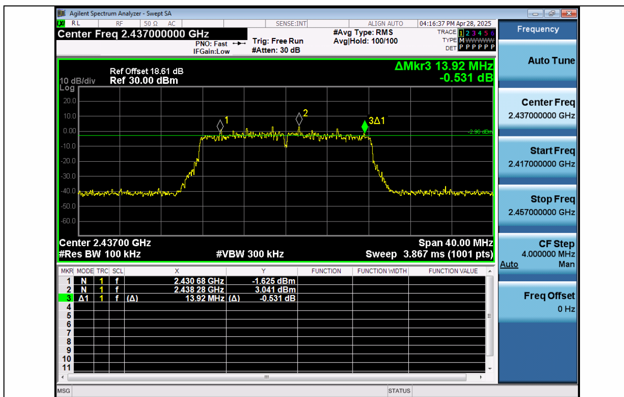
11G-Ant1-2437-PASS
