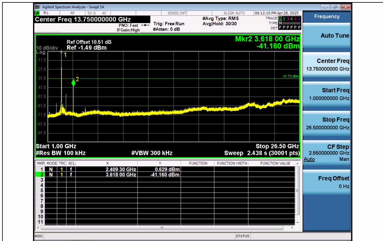
11AX20SISO-Ant1-2412-1000~26500-PASS
