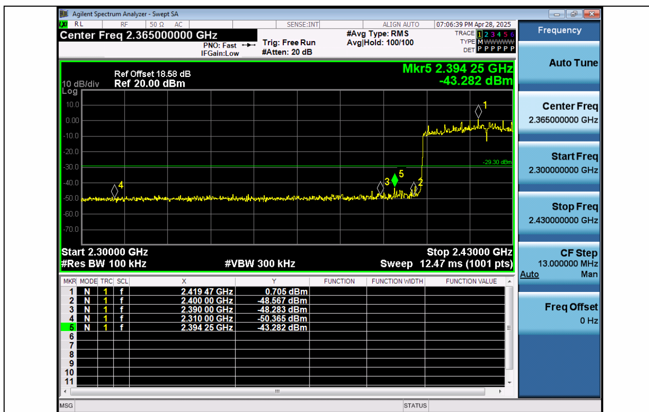
11AX40SISO-Ant1-2422-PASS
