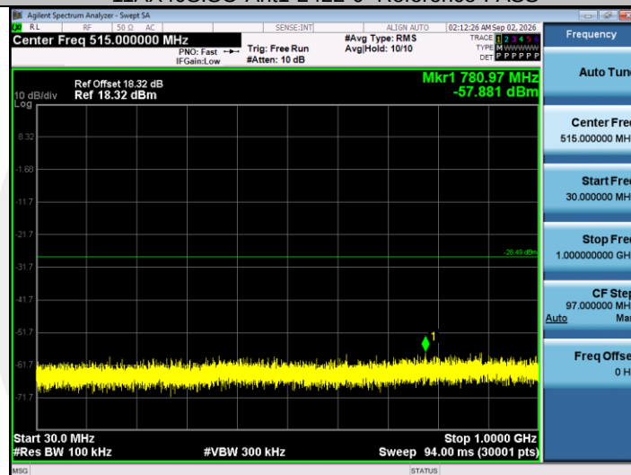
11AX40SISO-Ant1-2422-30~1000-PASS
