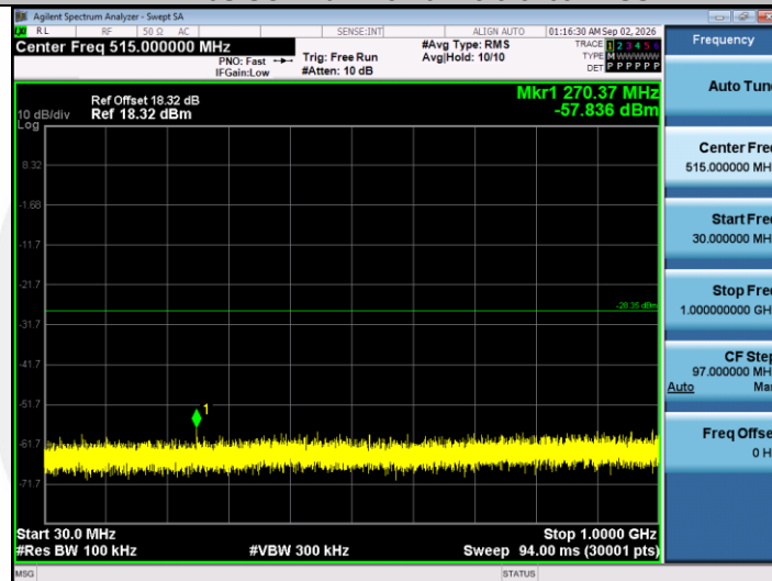
11N40SISO-Ant1-2452-30~1000-PASS
