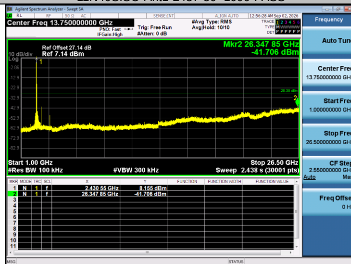
11N40SISO-Ant1-2437-1000~26500-PASS
