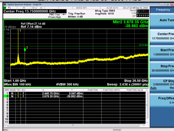
11N40SISO-Ant1-2452-1000~26500-PASS
