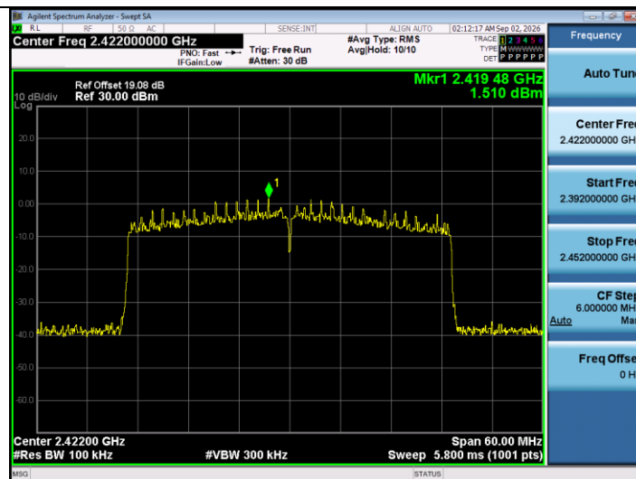
11AX40SISO-Ant1-2422-0~Reference-PASS
