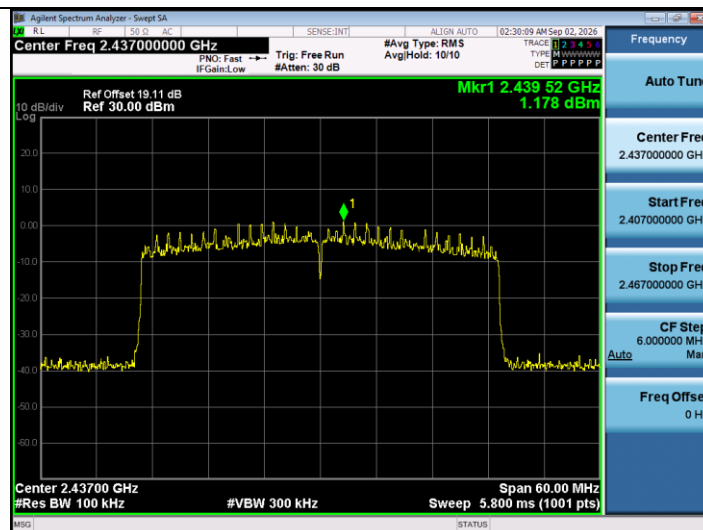
11AX40SISO-Ant1-2437-0~Reference-PASS
