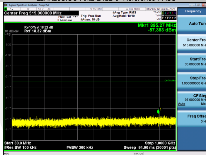
11AX20SISO-Ant1-2412-30~1000-PASS
