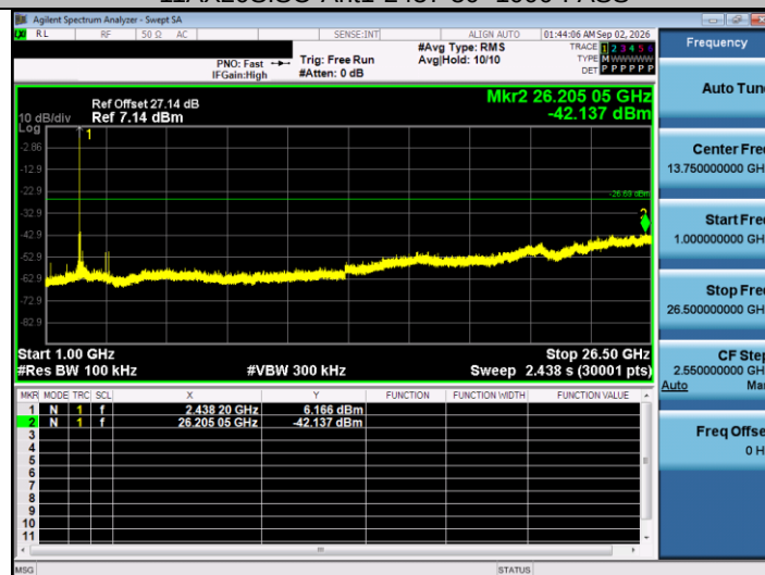
11AX20SISO-Ant1-2437-1000~26500-PASS
