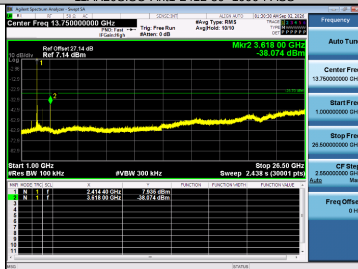
11AX20SISO-Ant1-2412-1000~26500-PASS
