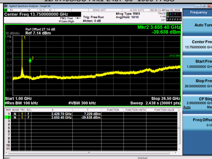
11AX40SISO-Ant1-2437-1000~26500-PASS
