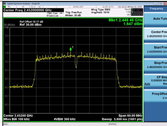
11N40SISO-Ant1-2452-0~Reference-PASS
