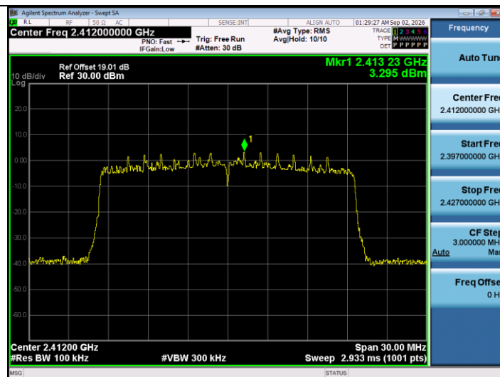
11AX20SISO-Ant1-2412-0~Reference-PASS
