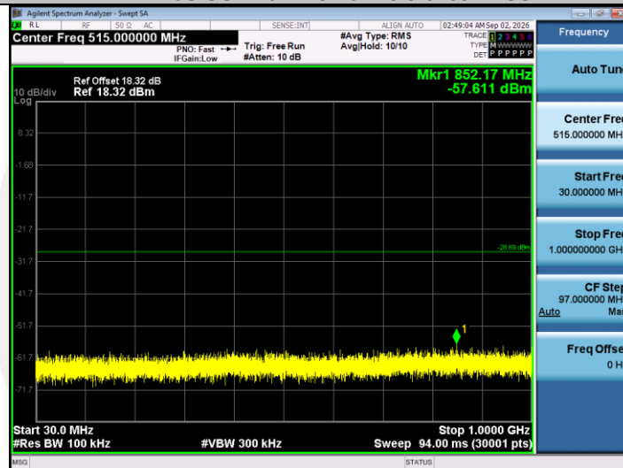
11AX40SISO-Ant1-2452-30~1000-PASS
