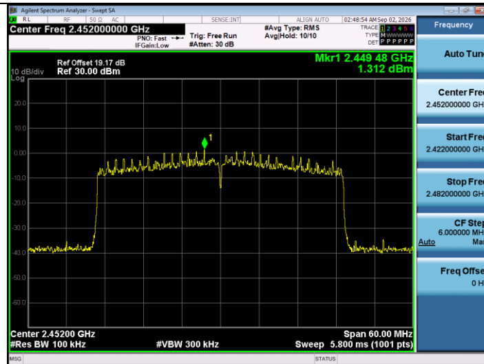
11AX40SISO-Ant1-2452-0~Reference-PASS
