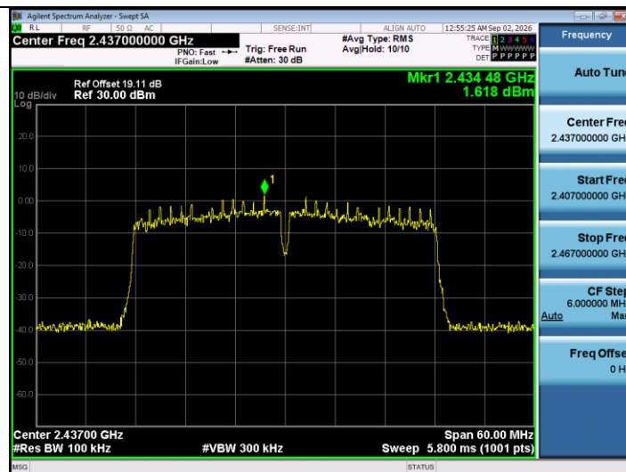
11N40SISO-Ant1-2437-0~Reference-PASS
