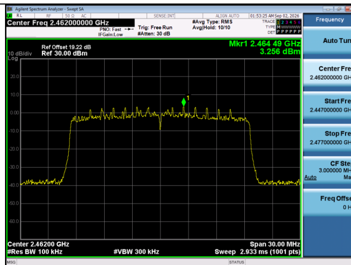
11AX20SISO-Ant1-2462-0~Reference-PASS
