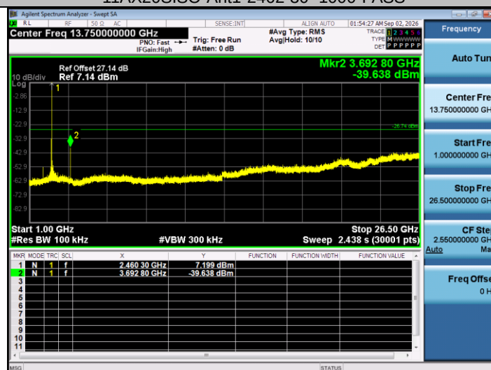
11AX20SISO-Ant1-2462-1000~26500-PASS
