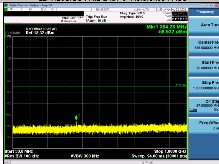
11AX20SISO-Ant1-2437-30~1000-PASS
