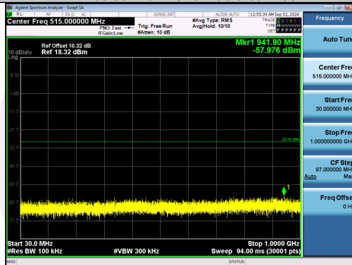
11N40SISO-Ant1-2437-30~1000-PASS
