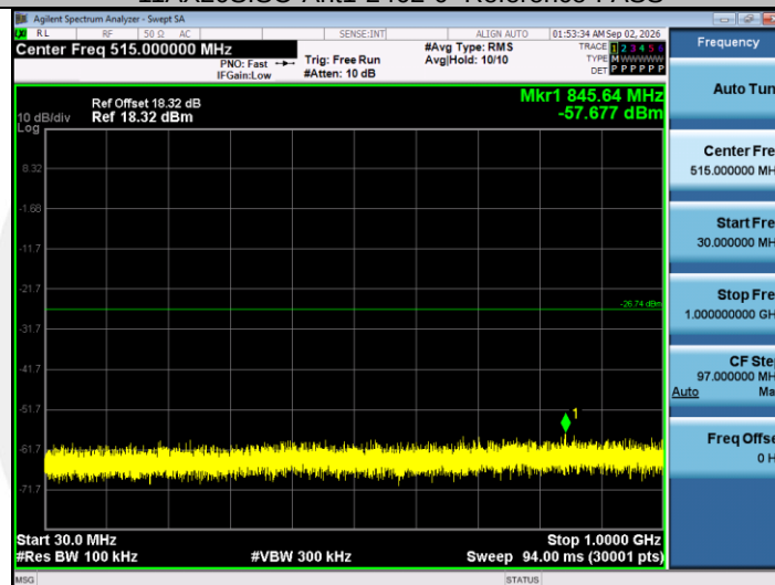
11AX20SISO-Ant1-2462-30~1000-PASS
