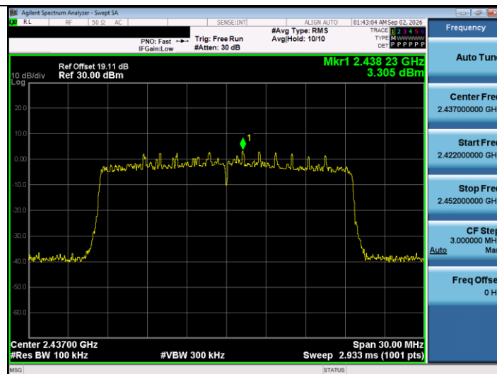
11AX20SISO-Ant1-2437-0~Reference-PASS
