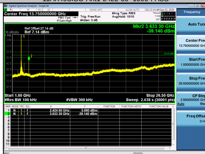
11AX40SISO-Ant1-2422-1000~26500-PASS
