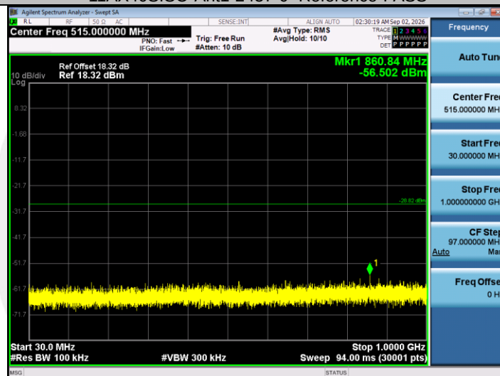
11AX40SISO-Ant1-2437-30~1000-PASS
