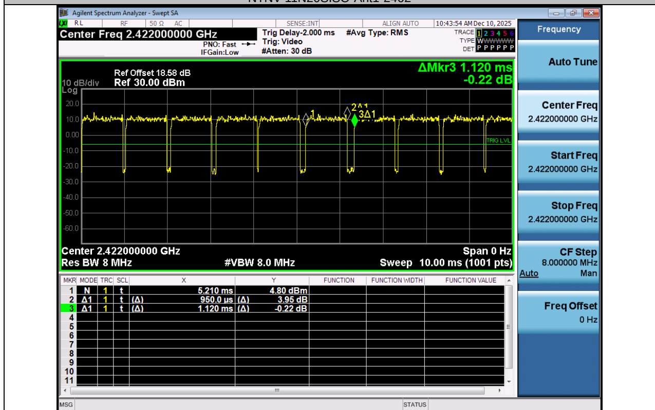
NTNV-11N40SISO-Ant1-2422
