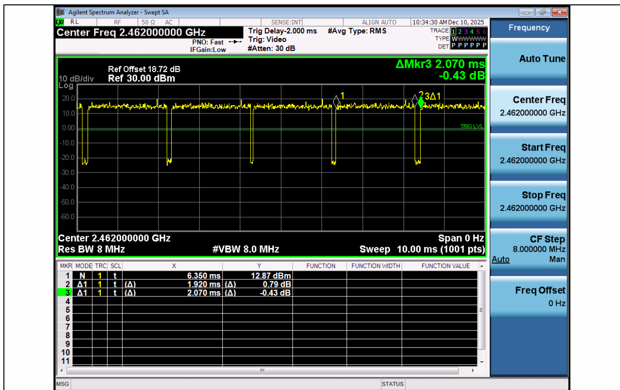
NTNV-11N20SISO-Ant1-2462
