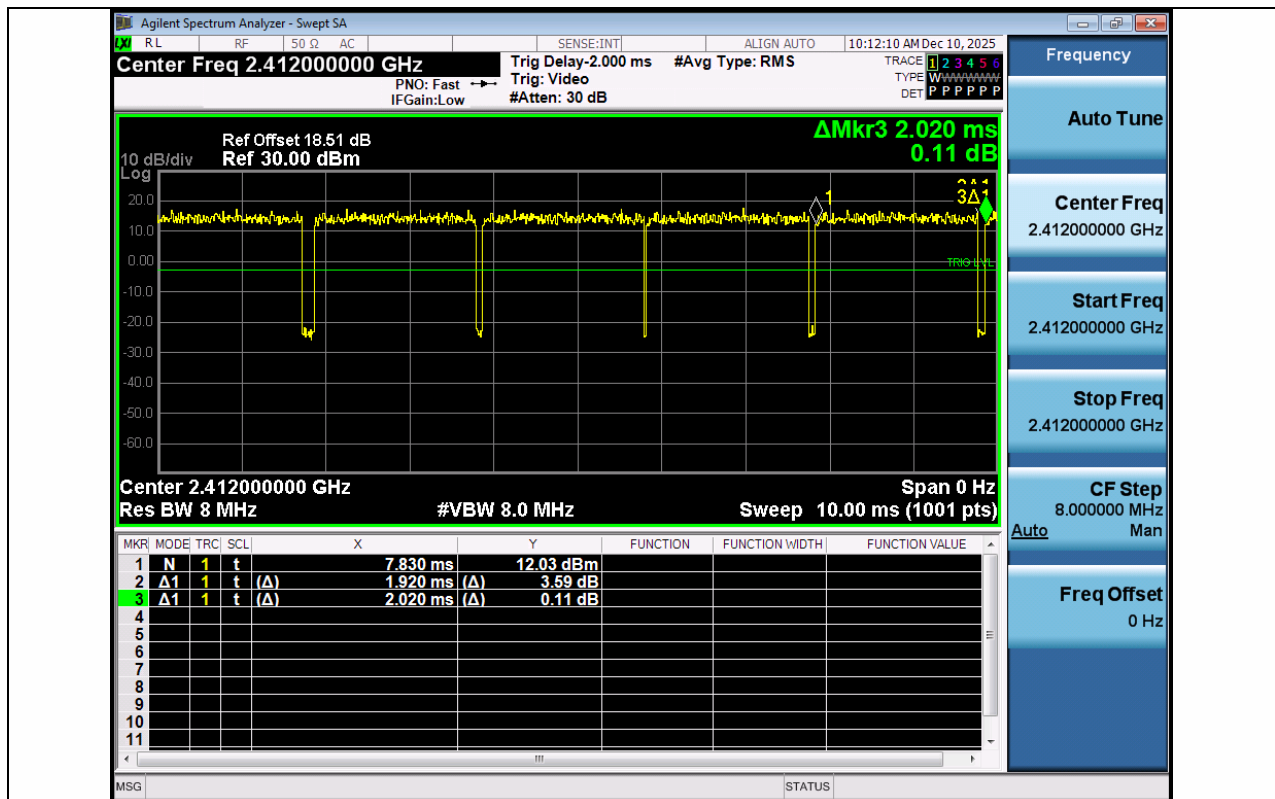
NTNV-11N20SISO-Ant1-2412
