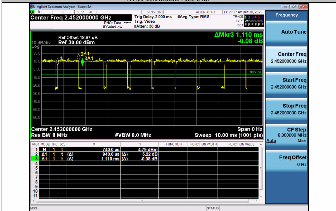
NTNV-11N40SISO-Ant1-2452
