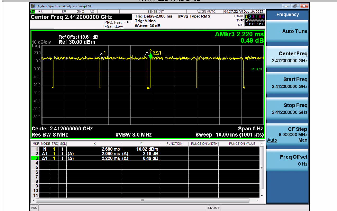
NTNV-11G-Ant1-2412
