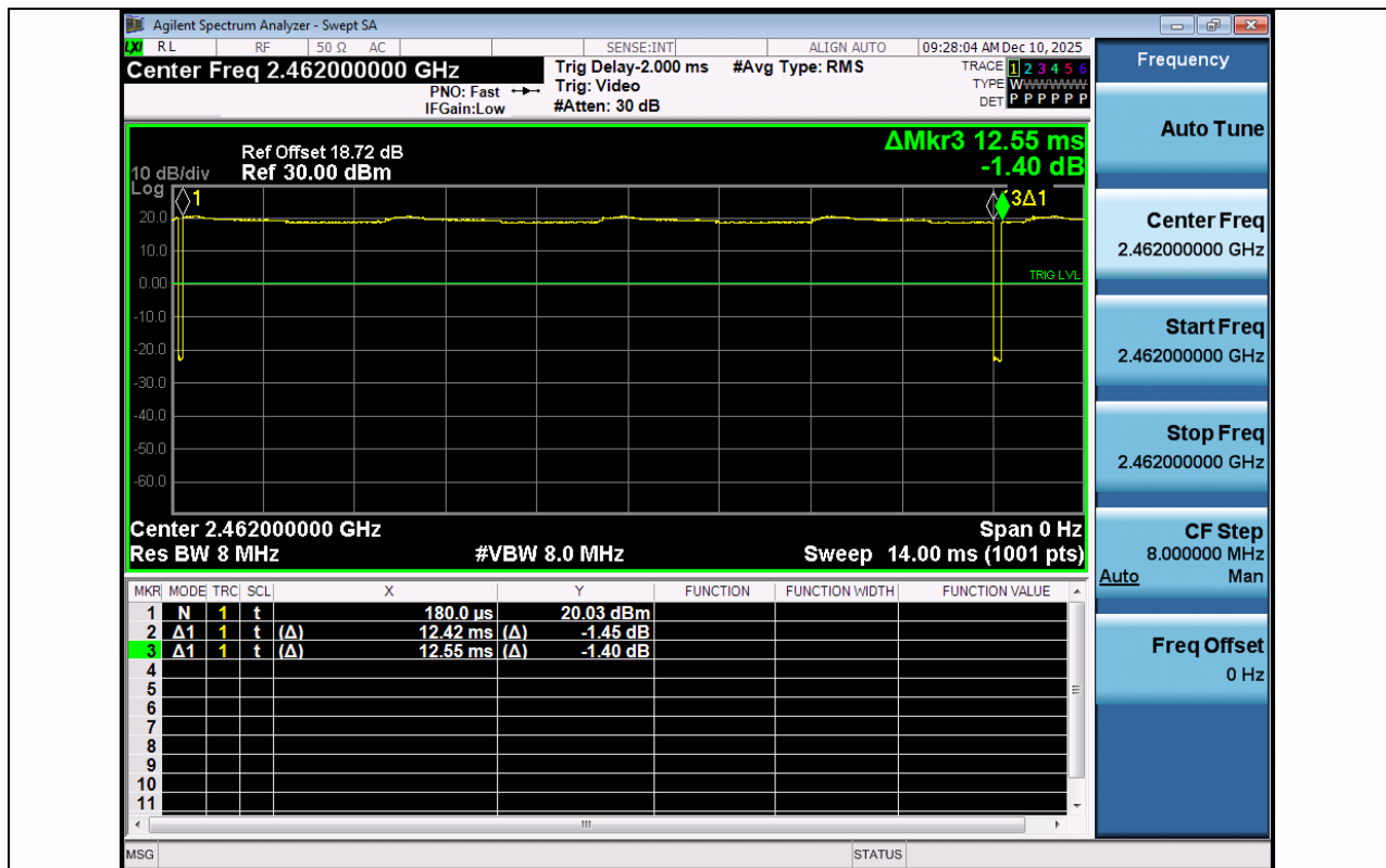
NTNV-11B-Ant1-2462
