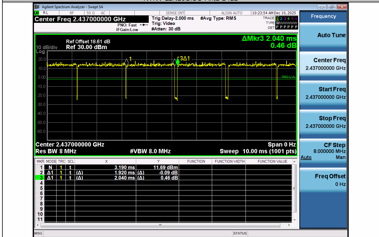
NTNV-11N20SISO-Ant1-2437
