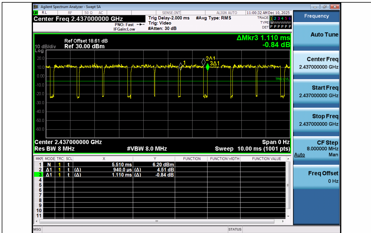
NTNV-11N40SISO-Ant1-2437
