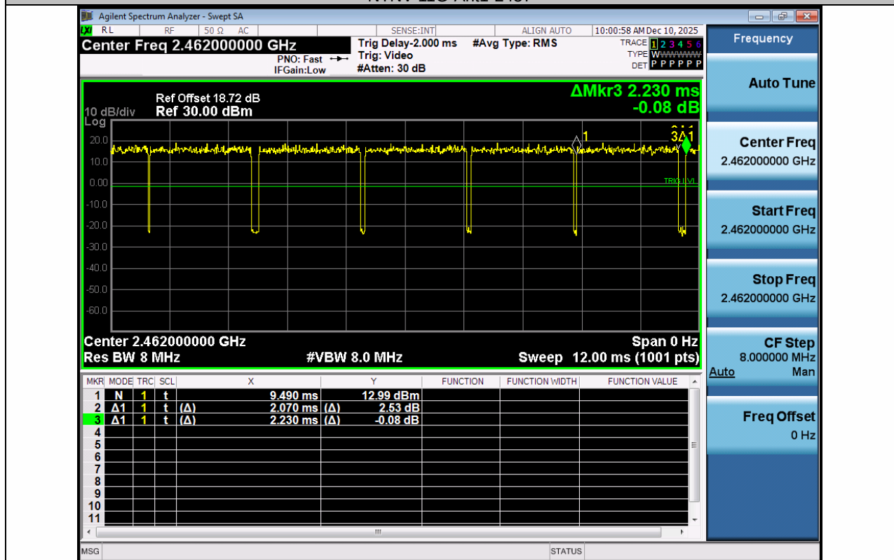
NTNV-11G-Ant1-2462
