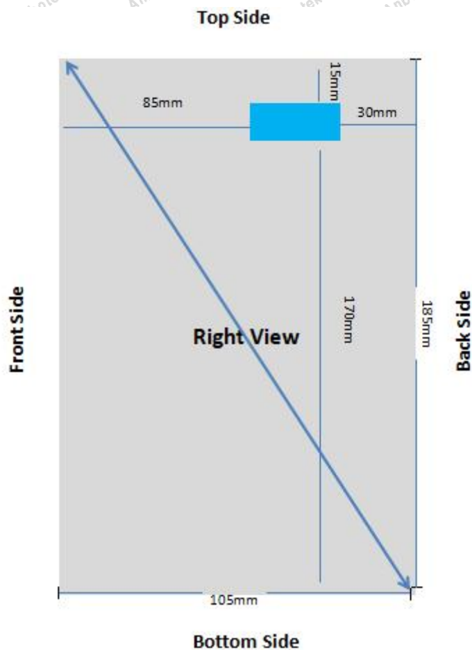
Positions for SAR tests; Body mode
