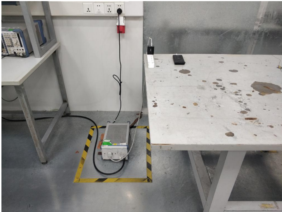
FCC ID: 2AOKB-A1617 Photo of Conducted Emission Measurement
