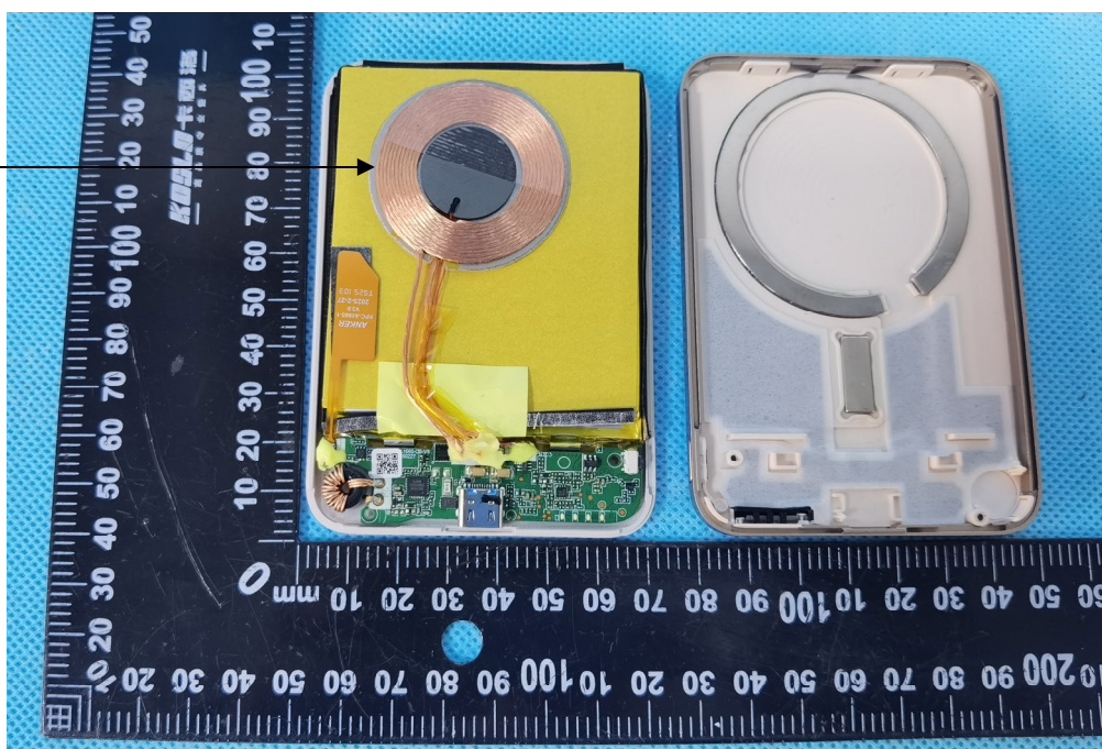
Coil Antenna
